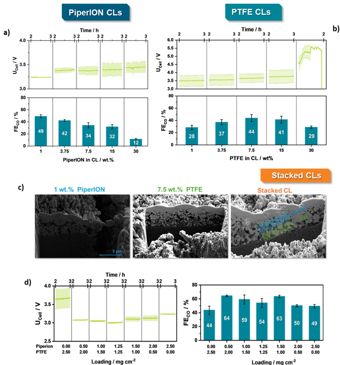
Fig. 3 Electrochemical characterization of the herein presented catalytic layers/GDEs at 300 \text{ mA cm}^{-2} at 60 \text{ }^\circ\text{C} between 2nd and 3rd hour of electrolysis for the PiperION-bound CLs (a), PTFE-bound (b) and stacked (d) CLs. FIB-SEM analysis of the different catalytic layers (c).
