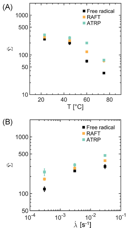
Fig. 4 Rate- and temperature-dependent damage of multiple-networks. The damage due to filler networks scission, \bar{\Sigma} (A) decreases with temperature and (B) increases with rate due to viscoelastic dissipation ahead of the crack. This observation indicates that dissipation mechanisms – viscoelasticity and damage – synergistically operate ahead of the crack. Under most loading conditions, filler networks synthesized by RAFT and ATRP suffer more damage compared to that made by free radical polymerization (FRP).
