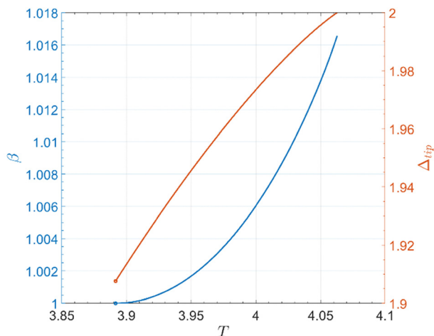
Fig. 8 Normalized crack length \beta (blue line) and \Delta A_{\text{tip}} (red line) versus normalized time T for \alpha = 1.2 < \alpha^* = 1.7071 . Simulations used \beta_0 = 1 , \eta_{\text{max}} = 1 , \phi_{\text{max}} = 2 .
