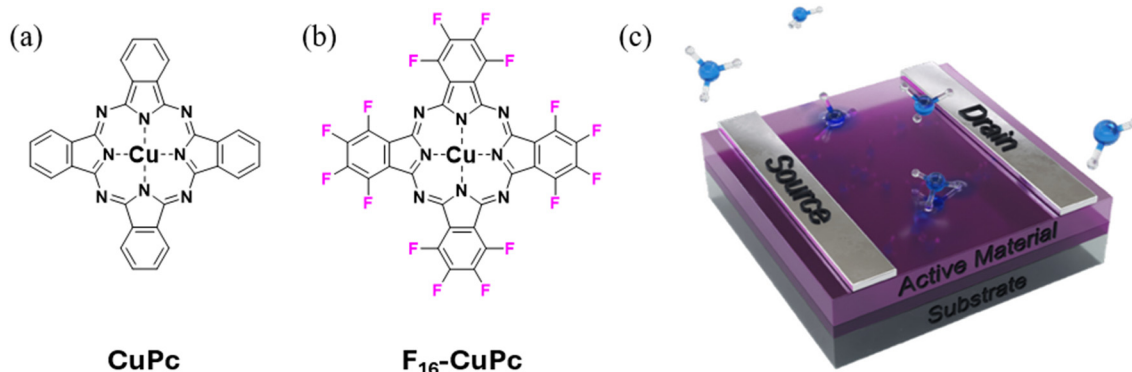
Fig. 1 Molecular structure of a) CuPc and b) \text{F}_{16}\text{CuPc} , and c) the OTFT sensor device scheme.
