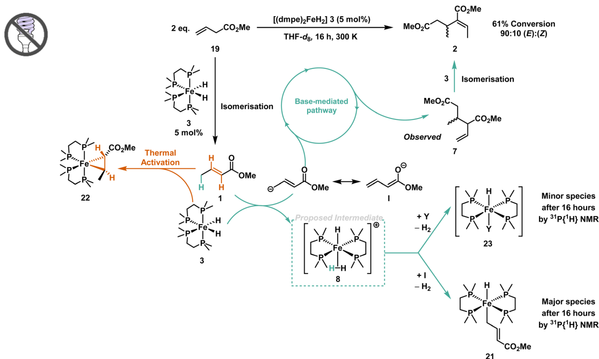
Scheme 2 Isomerisation of methyl 3-butenate 19 to methyl crotonate 1 by [(dmpe) 2 FeH 2 ] 3 . Methyl crotonate 1 can then be dimerised by the base-mediated pathway to give the dimer intermediate dimethyl 2-ethenyl-3-methylpentanedioate 7 which itself can be isomerised by [(dmpe) 2 FeH 2 ] 3 to give (E,Z)-2-ethylidene-3-methylpentanedioate 2 . 31 P NMR spectroscopic analysis of the reaction shows that the major iron species is trans -[(dmpe) 2 FeH(CH 2 CH=CHCO 2 Me)] 21 , with minor amounts of [(dmpe) 2 FeHY] 23 . Minor amounts of [(dmpe) 2 Fe(η 2 -1)] 22 by thermal activation of [(dmpe) 2 FeH 2 ] 3 were also observed.
