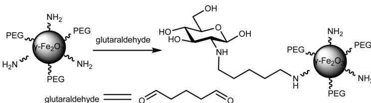
Fig. 8 Representative glyco-based magnetic nanocomposites with carbohydrates serving as targeting ligands. (a) Synthesis of glyco-grafted magnetic nanoparticles (MNPs) by amide bond formation between carboxylated glycans and aminated MNPs; (b) synthesis of Sialyl Lewis X -grafted MNPs by EDC/NHS coupling strategy; (c) synthesis of glucose-functionalized MNPs using a glutaraldehyde linker; (d) synthesis of sugar-coated MNPs by chemical adsorption.
