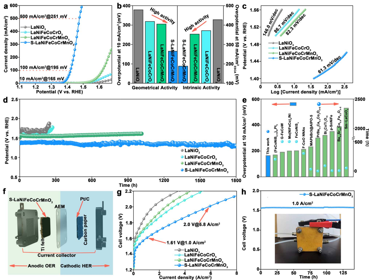
Fig. 2 Electrochemical performance evaluation of the S-LaNiFeCoCrMnO 3 catalyst toward the OER in 1.0 M KOH solution. (a) LSV curves of LaNiO 3 , LaNiFeCoCrO 3 , LaNiFeCoCrMnO 3 , and S-LaNiFeCoCrMnO 3 catalysts. (b) Comparison of geometric and ECSA-normalized activity for LaNiO 3 , LaNiFeCoCrO 3 , LaNiFeCoCrMnO 3 , and S-LaNiFeCoCrMnO 3 catalysts. (c) Tafel slopes of LaNiO 3 , LaNiFeCoCrO 3 , LaNiFeCoCrMnO 3 , and S-LaNiFeCoCrMnO 3 catalysts. (d) Chronopotentiometric curves of LaNiO 3 , LaNiFeCoCrO 3 , LaNiFeCoCrMnO 3 , and S-LaNiFeCoCrMnO 3 catalysts at 10 mA cm -2 . (e) Comparison of S-LaNiFeCoCrMnO 3 and previously reported catalysts for perovskite oxides and sulfides. (f) Schematic diagram to illustrate the anodic oxygen evolution and cathodic hydrogen evolution in AEMWEs. (g) Polarization curves of LaNiO 3 , LaNiFeCoCrO 3 , LaNiFeCoCrMnO 3 , and S-LaNiFeCoCrMnO 3 as anode catalysts in an anion exchange membrane water electrolyzer. (h) Chronopotentiometric curve of S-LaNiFeCoCrMnO 3 as an anode catalyst at 1.0 A cm -2 in an AEMWE.
