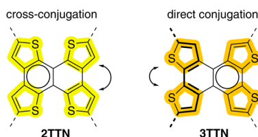
Scheme 1 (a) Thiophene-containing linkers and nodes used in reported COFs. (b) New isomeric naphthotetrathienophene (TTN) nodes reported here.
