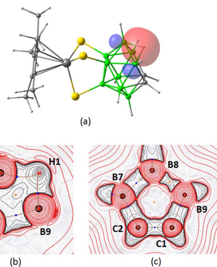
Fig. 8 (a) Selected NBO of 5 showing the 3c–2e interaction of B8–H1–B9 (isocontour values: \pm 0.045 [e bohr ^{-3/2} ]). Contour-line diagram of the Laplacian of the electron density along (b) B8–H1–B9 and (c) B7–B8–B9 planes in 5 .
