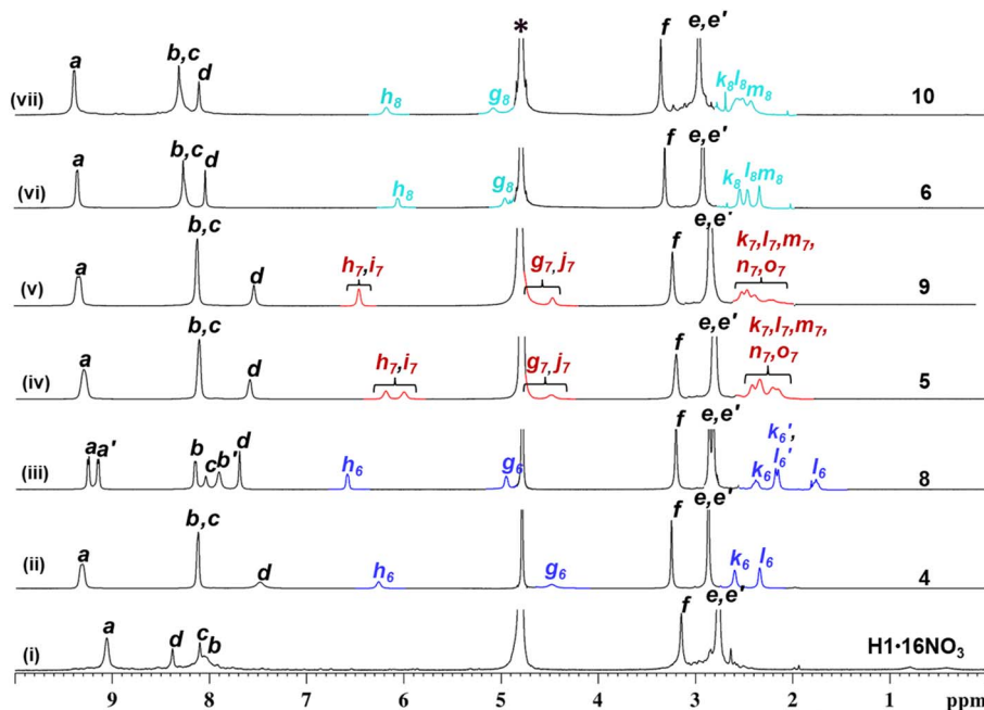
Fig. 6 ^1\text{H} NMR spectra (400 MHz, \text{D}_2\text{O} , 298 K, i.e., 25 ^\circ\text{C} ) for isolated samples of (i) \text{H1}\cdot 16\text{NO}_3 , (ii) [(\text{H6})_2\cdot\text{C(H1)}]\cdot 16\text{NO}_3 (4), (iii) [\{\text{G}\cdot(\text{H6})_2\}\cdot\text{C(H1)}]\cdot 17\text{NO}_3 (8), (iv) [(\text{H7})_2\cdot\text{C(H1)}]\cdot 16\text{NO}_3 (5), (v) [\{\text{G}\cdot(\text{H7})_2\}\cdot\text{C(H1)}]\cdot 17\text{NO}_3 (9), (vi) [(\text{H8})_2\cdot\text{C(H1)}]\cdot 16\text{NO}_3 (6), and (vii) [\{\text{G}\cdot(\text{H8})_2\}\cdot\text{C(H1)}]\cdot 17\text{NO}_3 (10).
