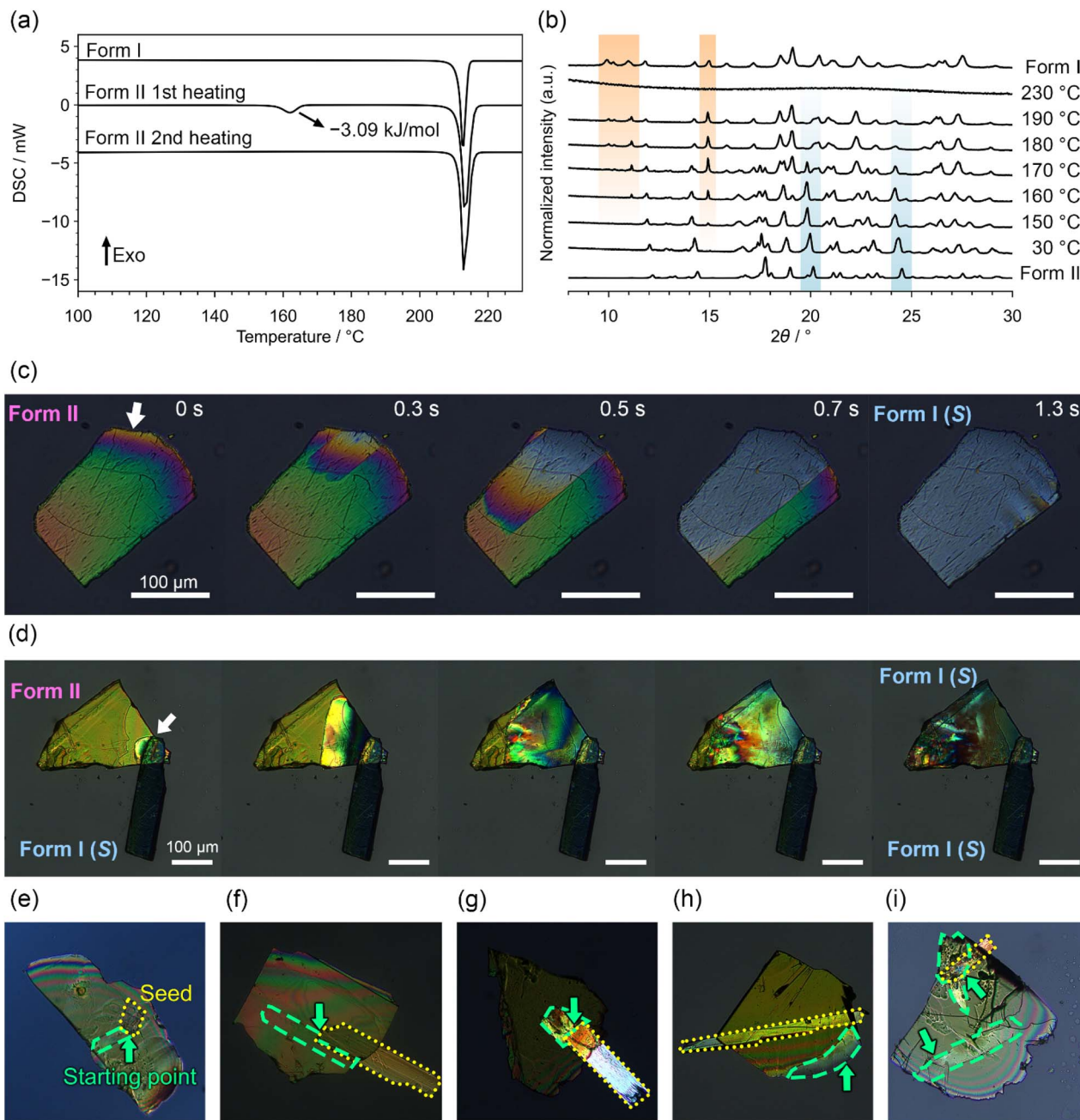
Fig. 3 (a) DSC curves for forms I and II. The thermograms for form I and the second heating of form II are plotted with a vertical offset of 4 mW for clarity. The heating rate was 5 K \text{min}^{-1} . (b) VT-PXRD patterns for form II. The observed patterns for forms I and II are indicated. The orange and blue shaded regions indicate the characteristic peaks for forms I and II, respectively. (c) POM images during the SC-SC structural transformation from form II to I at 180 °C. The scale bar represents 100 \mu\text{m} . (d) POM images during chirality transfer from form I to II by solid-seeding at 150 °C. (e-g) POM images of typical progression behaviour when the transition started from the contact point. Areas with yellow frames indicate a seed crystal. The arrows indicate the starting point of the transition. Areas with green frames indicate where the transition occurred. (h) POM image during the transition initiated from the edge of the crystal. (i) POM image during the transition initiated from multiple points.
