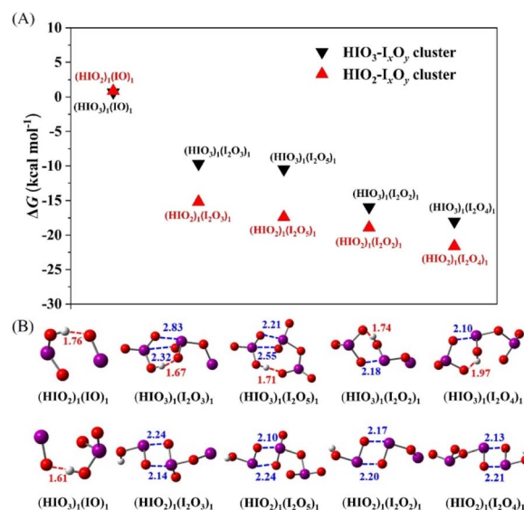
Fig. 1 Formation free energy ( \Delta G ) (A) and global minimum configurations (B) of \text{I}_x\text{O}_y\text{-HIO}_{2-3} dimers at the DLPNO-CCSD(T)/aug-cc-pVTZ(-PP)//M06-2X/aug-cc-pVTZ(-PP) level of theory at 298.15 K. The red balls represent oxygen atoms, purple ones are for iodine atoms, and white ones are for hydrogen atoms. The red dashed lines in the configurations represent hydrogen bonds (HBs), and the blue dashed lines represent XBs. The red and blue numbers indicate the bond lengths of HBs and XBs, respectively. The bond lengths are given in Å.
