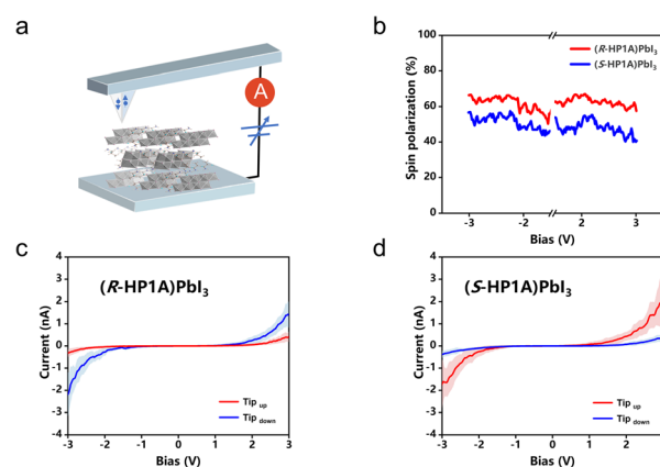
Fig. 5 (a) Schematic representation of the mCP-AFM measurements. (b) Average values of spin polarization in ( R -HP1A)PbI 3 (red) and ( S -HP1A)PbI 3 (blue). (c and d) Room-temperature mCP-AFM measurements for ( R/S -HP1A)PbI 3 . The shaded region around the lines marks the standard deviation for the average results.
