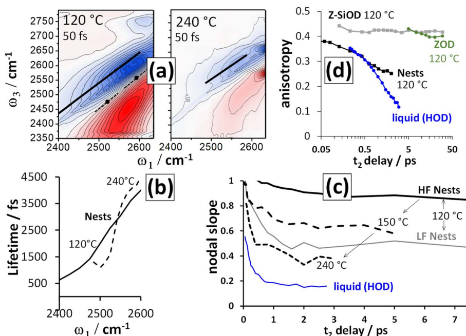
Fig. 4 Lifetime, spectral diffusion and anisotropy decays of the ZSM-5 silanol nests. (a) 2D-IR spectra of ZSM-5 in flowing N 2 /D 2 O vapour were collected at 120 °C and 240 °C (<XXYY> polarisation, t_2 \sim 50 fs). (b) The spectra in (a) are analysed as a function of waiting time t_2 by single exponential fitting. (c) Spectral diffusion (nodal slope) around two different \omega_1 values at three temperatures. (d) anisotropy decays calculated from the positive ESA bands for the 120 °C measurement using both <XXXX> and <XXYY> data. In (a), the positions where lifetimes and nodal slopes were determined are indicated by solid and dotted lines. Shown for comparison in (c) and (d) are measurements of room temperature liquid HOD in H 2 O and (d) free silanol and the Brønsted site.
