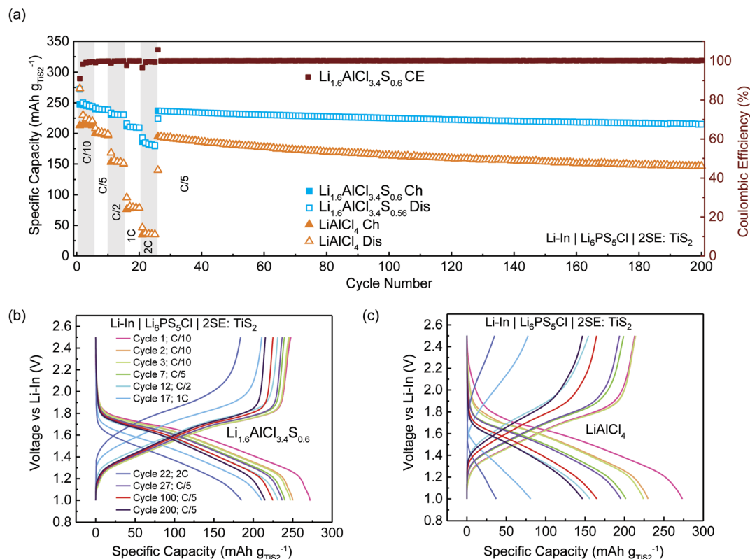
Fig. 5 Galvanostatic cycling of 2SE: \text{TiS}_2 catholyte with argyrodite \text{Li}_6\text{PS}_5\text{Cl} as the separator. (a) Rate performance of \text{Li–In} | \text{Li}_6\text{PS}_5\text{Cl} | 2\text{SE:TiS}_2 cell (SE = \text{LiAlCl}_4 or \text{Li}_{1.6}\text{AlCl}_{3.4}\text{S}_{0.6} ) followed by long-term cycling at C/5, where C = 239\text{ mA h g}^{-1} . Voltage profile of cycle 1 along with the 2nd cycles of each C-rate for a (b) \text{Li–In} | \text{Li}_6\text{PS}_5\text{Cl} | 2(\text{Li}_{1.6}\text{AlCl}_{3.4}\text{S}_{0.6}):\text{TiS}_2 cell and (c) \text{Li–In} | \text{Li}_6\text{PS}_5\text{Cl} | 2(\text{LiAlCl}_4):\text{TiS}_2 cell.
