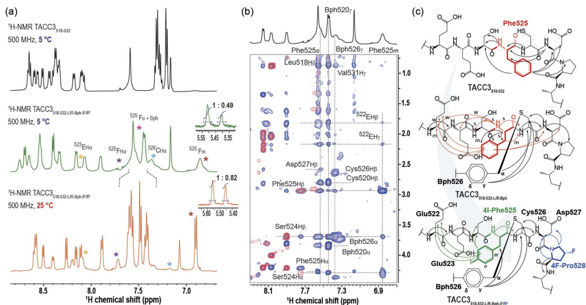
Fig. 4 NMR secondary structure analysis of TACC3 518-532 and constrained TACC3 518-532-L/R-Bph-LR-IF/FP . (a) 1 H-NMR spectra of TACC3 518-532 (in black) and TACC3 518-532-L/R-Bph-IF/FP (in green) showing the amide-bond region of the peptides as observed at 5 °C; shown in orange is the 1 H-NMR spectra of TACC3 518-532-L/R-Bph-IF/FP as observed at 25 °C; (b) superposition of the 1 H– 1 H TOCSY (in red) and 1 H– 1 H NOESY spectra (in blue) at the NH–H \alpha region of constrained TACC3 518-532-L/R-Bph-IF/FP ; (c) schematics showing the comparative intramolecular spatial 1 H– 1 H NOESY contacts and the phenylalanine aromatic ring orientation as observed within TACC3 518-532 WT, control constrained TACC3 518-532-L/R-Bph and TACC3 518-532-L/R-Bph-LR-IF/FP . All samples as measured in buffer/D 2 O 90/10% vol/vol. Buffer: 25 mM potassium phosphate, 50 mM NaCl, 5 mM MgCl 2 , pH = 7.5.
