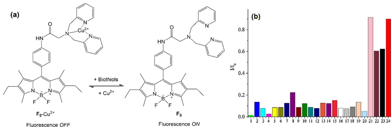
Fig. 11 (a) Sensing mechanism of F_5\text{-Cu}^{2+} for biothiols, and (b) fluorescence changes of (1) F_5\text{-Cu}^{2+} upon the addition of (2–20) other amino acids, (21) \text{Na}_2\text{S} , (22) Cys, (23) Hcy, and (24) GSH, 53 adapted from ref. 53, C.-C. Zhao, Y. Chen, H.-Y. Zhang, B.-J. Zhou, X.-J. Lv and W.-F. Fu, J. Photochem. Photobiol. A Chem. , 2014, 282 , 41–46. Copyright 2014, with permission from Elsevier.
