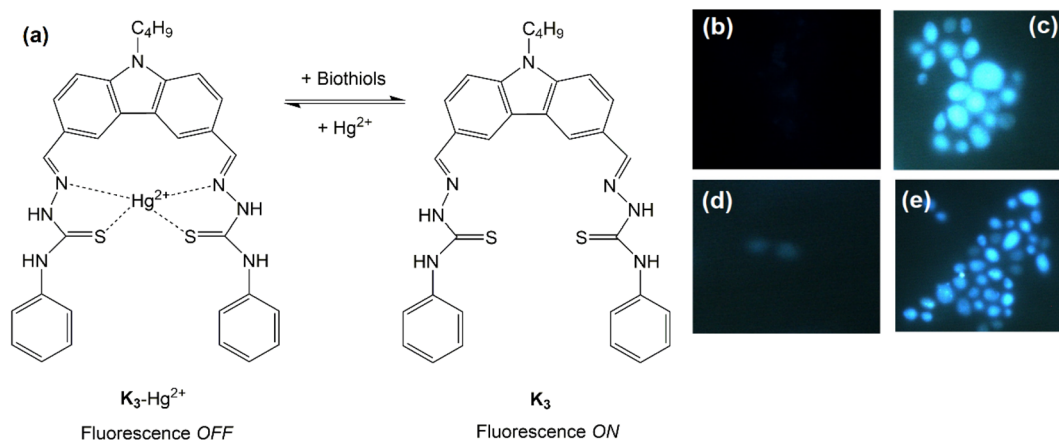
Fig. 31 (a) \text{K}_3\text{-Hg}^{2+} sensor for biothiols, (b–e) fluorescence microscopy images: (b) Candida albicans cells only, (c) Candida albicans + \text{K}_3 , (d) Candida albicans + \text{K}_3\text{-Hg}^{2+} , (e) Candida albicans + \text{K}_3\text{-Hg}^{2+} + Cys, 83 adapted from ref. 83, A. K. Mahapatra, J. Roy, P. Sahoo, S. K. Mukhopadhyay, A. Banik and D. Mandal, Tetrahedron Lett. , 2013, 54, 2946–2951. Copyright 2013, with permission from Elsevier.
