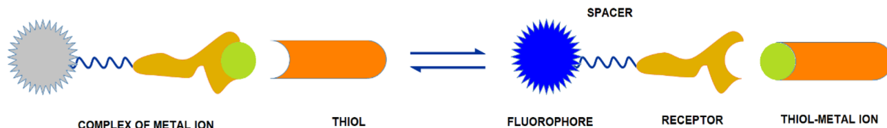
Fig. 1 The operating mechanism of the metal complexes as fluorescent sensors for detecting thiols based on the metal ion complexation/decomplexation reactions.
