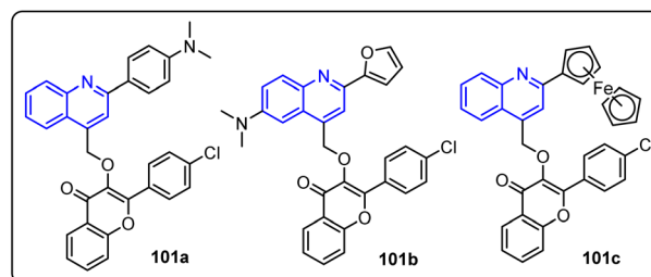
Scheme 23 Synthesis of quinolin-4-yl-methoxychromen-4-ones 101 .
