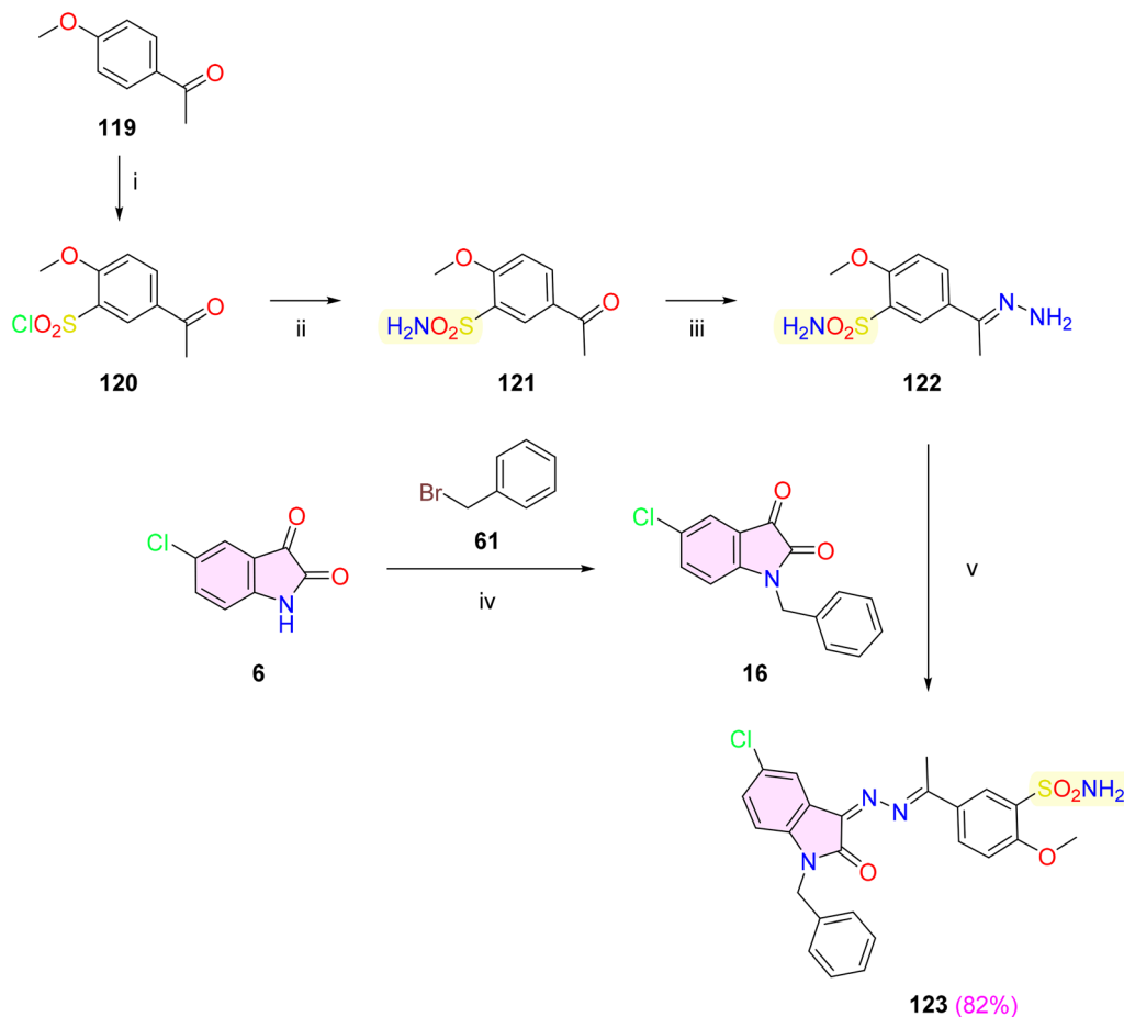
Scheme 20 Synthesis of isatin–sulphonamide hybrid 123 . Reagents and conditions: (i) HOSO 2 Cl, SOCl 2 , 0 °C, 30 min, r.t., 26 h; (ii) EtOH, ammonia, r.t.; (iii) N 2 H 4 ·H 2 O, EtOH, gl. AcOH (cat.) reflux, 4 h; (iv) K 2 CO 3 , MeCN, reflux, 5 h; (v) EtOH, gl. AcOH (cat.), reflux, 4 h.
