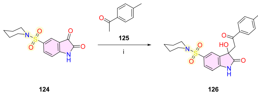
Scheme 21 Synthesis of isatin–sulphonamide hybrid 126 . Reagents and conditions: (i) EtNH 2 , MeOH.
