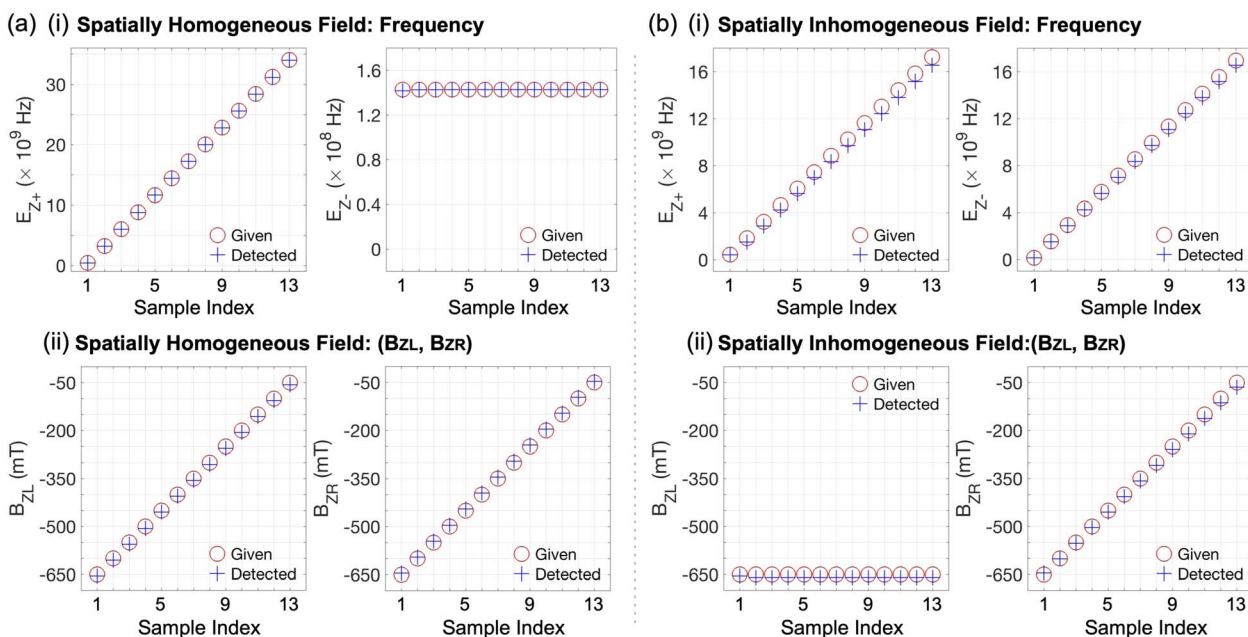
Fig. 5 (a) Performance of the DQD sensing protocol when the sensing target is constant (spatially homogeneous). Being secured with B_{ZL} ( =B_{ZR} ) ( =B_{ZL} = B_{ZR} ) that varies from -650 mT to -50 mT with an incremental step of 50 mT, simulation results well confirm the operational feasibility of the sensing protocol, so the inaccuracies of E_{Z+} 's & E_{Z-} 's derived from simulated |\psi_M\rangle are just 0.49 \pm 0.83\% & 0.090 \pm 0.21\% of their theoretical values, and, accordingly, the detected B_{ZL} 's & B_{ZR} 's deviate by -5.72 \pm 0.47 mT and 4.49 \pm 0.46 mT from their given quantities, respectively. (b) Computational results driven with spatially inhomogeneous B_{Z(External)} that is considered with B_{ZL} = -650 mV and B_{ZR} varying from -650 mT to -50 mT with a step of 50 mV. As similarly to the case of homogeneous targets, detected values here solidly follow given quantities. While the accuracies generally become worse than the case of homogeneous targets ( E_{Z+} 's: 6.70 \pm 3.81\% , E_{Z-} 's: 2.20 \pm 0.41\% , B_{ZL} 's: -10.02 \pm 1.35 mT, and B_{ZR} 's: -7.00 \pm 5.27 mT), simulation results are fair enough to claim the operational feasibility of the protocol under inhomogeneous sensing targets.
