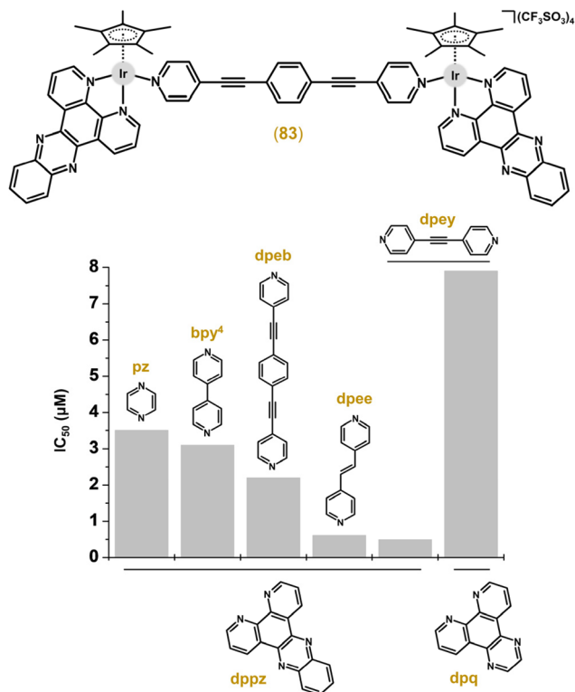
Fig. 19 The structural formulas of the representative dinuclear complex [\text{Ir}_2(\mu\text{-dpeb})(\eta^5\text{-Cp}^*)_2(\text{dppz})_2](\text{CF}_3\text{SO}_3)_4 ( 83 ; top) and its poly-pyridyl analogues, given with a comparison of their in vitro antiproliferative activity against MCF-7 breast carcinoma cells.
