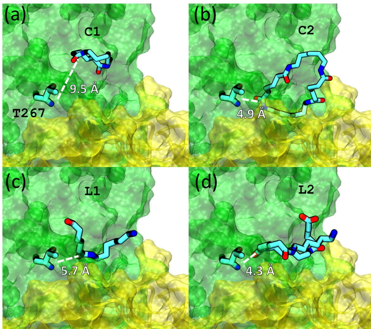
Fig. 3 MD simulated binding of Nylon-6,6 substrates with C1 (a), C2 (b), L1 (c), and L2 (d). Nylon-6,6 is shown in stick, with chain A in green and chain D in yellow. Chains B and C are omitted for clarity. The catalytic residue T267 and Nylon-6,6 substrates are in stick. Distances between T267 and carbonyl carbon of Nylon-6,6 substrates are labeled. Note the close proximity of C2 and L2 to T267. The snapshots are taken from the last conformations of 5 ns trajectories.
