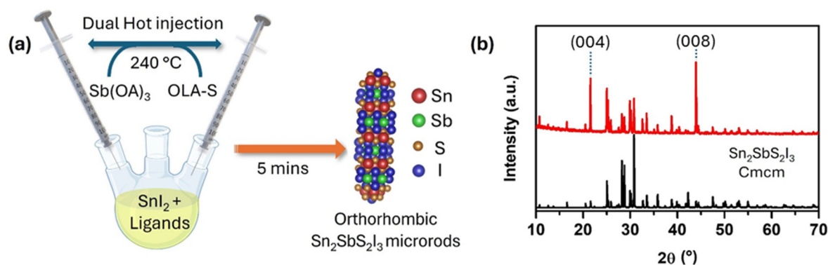
Fig. 1 (a) Scheme of the colloidal dual hot-injection protocol for Sn 2 SbS 2 I 3 microrods synthesis; (b) XRD spectra of the as-synthesised Sn 2 SbS 2 I 3 microrods (red) and the Sn 2 SbS 2 I 3 Cmcm reference (ICSD number 23344).
