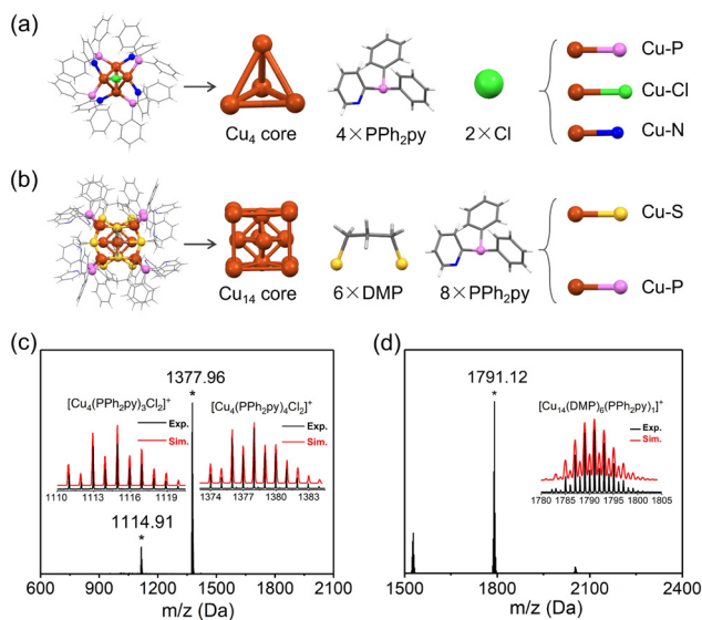
Fig. 1 Structural anatomy of (a) \text{Cu}_4 and (b) \text{Cu}_{14} nanoclusters. Positive-mode ESI-MS spectrum of (c) \text{Cu}_4 and (d) \text{Cu}_{14} nanoclusters. Insets: isotope patterns of experimental (black) and simulated (red) spectra of corresponding nanoclusters. Color legend: brown = Cu; yellow = S; pink = P; green = Cl; blue = N. For clarity, C and H atoms are shown in wireframe mode.
