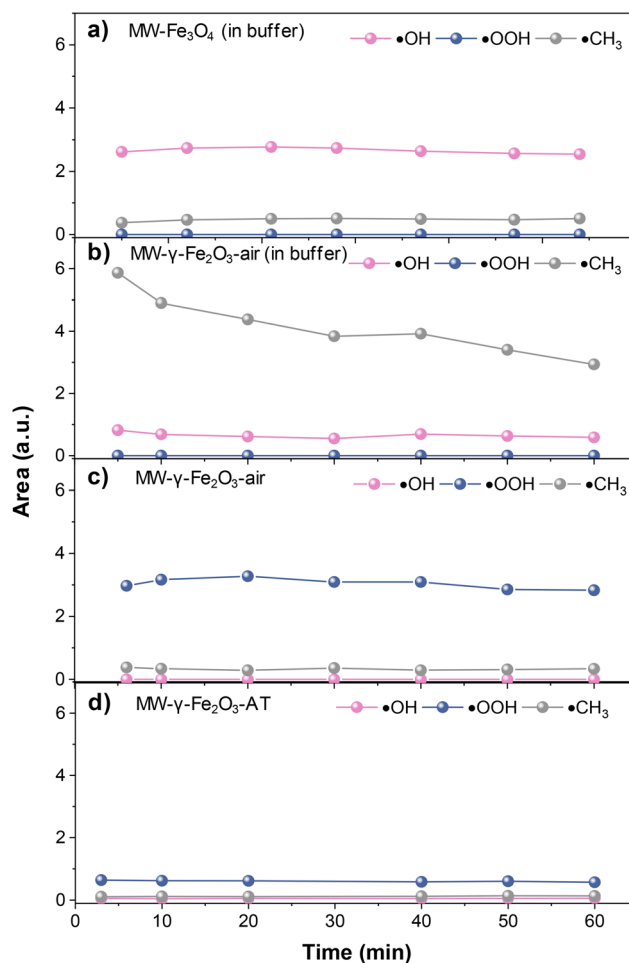
Fig. 4 Effect of the buffer and the oxidation of the NPs on the free radical formation measured at pH = 4.8. (a) \text{Fe}_3\text{O}_4 in buffer, (b) MW- \gamma\text{-Fe}_2\text{O}_3 -air in buffer, (c) MW- \gamma\text{-Fe}_2\text{O}_3 -air measured without buffer and (d) MW- \gamma\text{-Fe}_2\text{O}_3 oxidized by an acidic treatment (AT) measured without buffer.
