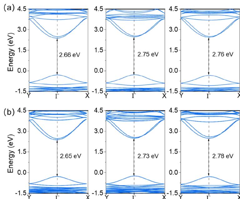
Fig. 3 Band structures (calculated using HSE06) of (a) monolayer and (b) bilayer RP-phase (\text{PMA})_2\text{PbI}_4 , (\text{THMA})_2\text{PbI}_4 and (\text{FUMA})_2\text{PbI}_4 perovskites.
