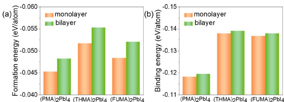
Fig. 2 (a) Formation energy ( \Delta H_{\text{form}} ) and (b) binding energy ( E_{\text{B}} ) of three RP-phase (\text{PMA})_2\text{PbI}_4 , (\text{THMA})_2\text{PbI}_4 and (\text{FUMA})_2\text{PbI}_4 perovskites in the monolayer and bilayer forms.
