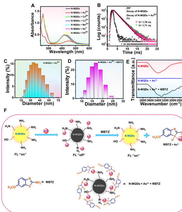
Fig. 7 (A) UV-vis absorbance spectra of N-MQDs before and after the addition of different lifetime analytes, showing a noticeable change for \text{As}^{3+} . (B) Fluorescence lifetime decay of the N-MQDs with and without treatment with \text{As}^{3+} . Hydrodynamic diameter of (C) \text{As}^{3+} -incubated N-MQDs solution and (D) MBTZ-incubated N-MQDs- \text{As}^{3+} system. (E) FT-IR spectra of N-MQDs after addition of \text{As}^{3+} and MBTZ. (F) Possible "on-off-on" mechanism of the N-MQDs after treatment with \text{As}^{3+} and MBTZ.
