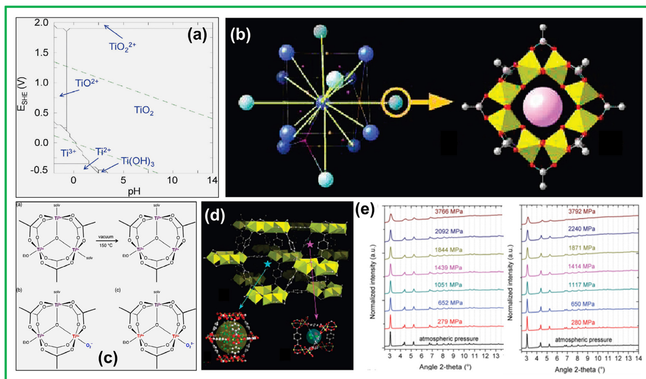
Fig. 1 (a) Pourbaix diagrams of titanium calculated for [Ti^{4+}] = 10^{-3} \text{ mol L}^{-1} at 25 °C using the Hydra and Medusa software. Green dashed lines: O_2/H_2O and H_2O/H_2 redox couples. Reprinted with permission from ref. 67. Copyright 2017 The Royal Society of Chemistry. (b) The perspective view of a centered cubic (cc) arrangement and the 12-fold coordination is shown by yellow lines. Purple and orange dots indicate the positions of the centers of the tetrahedral and octahedral vacancies and the view of the perforated cyclic octamer with edge- and corner-sharing Ti octahedra; it corresponds to the atom with an orange circle of the classical cc packing through the SBU augmentation. Reprinted with permission from ref. 47. Copyright 2009 American Chemical Society. (c) Illustration of the proposed composition of the Ti_3O clusters in 1 after heating at 150 °C under vacuum, reacting with O_2 to form titanium(IV) superoxide, and reacting with O_2 to form titanium(IV) peroxide. Reprinted with permission from ref. 69. Copyright 2015 American Chemical Society. (d) Perspective view of MIL-125 with the central octamer surrounded by 12 others; the pink and blue stars indicate the centers of the tetrahedral and octahedral vacancies in MIL-125, ball and stick representation of the octahedral vacancy, filled by water molecules (in green); the large yellow sphere represents the effective, accessible volume of the cage, and the tetrahedral vacancy. Reprinted with permission from ref. 47. Copyright 2009 American Chemical Society. (e) Powder X-ray diffraction patterns ( \lambda = 0.694120 \text{ \AA} ) were obtained for MIL-125(Ti) and NH_2 -MIL-125(Ti) as a function of the applied pressure at room temperature. Reprinted with permission from ref. 70. Copyright 2015 The Royal Society of Chemistry.
