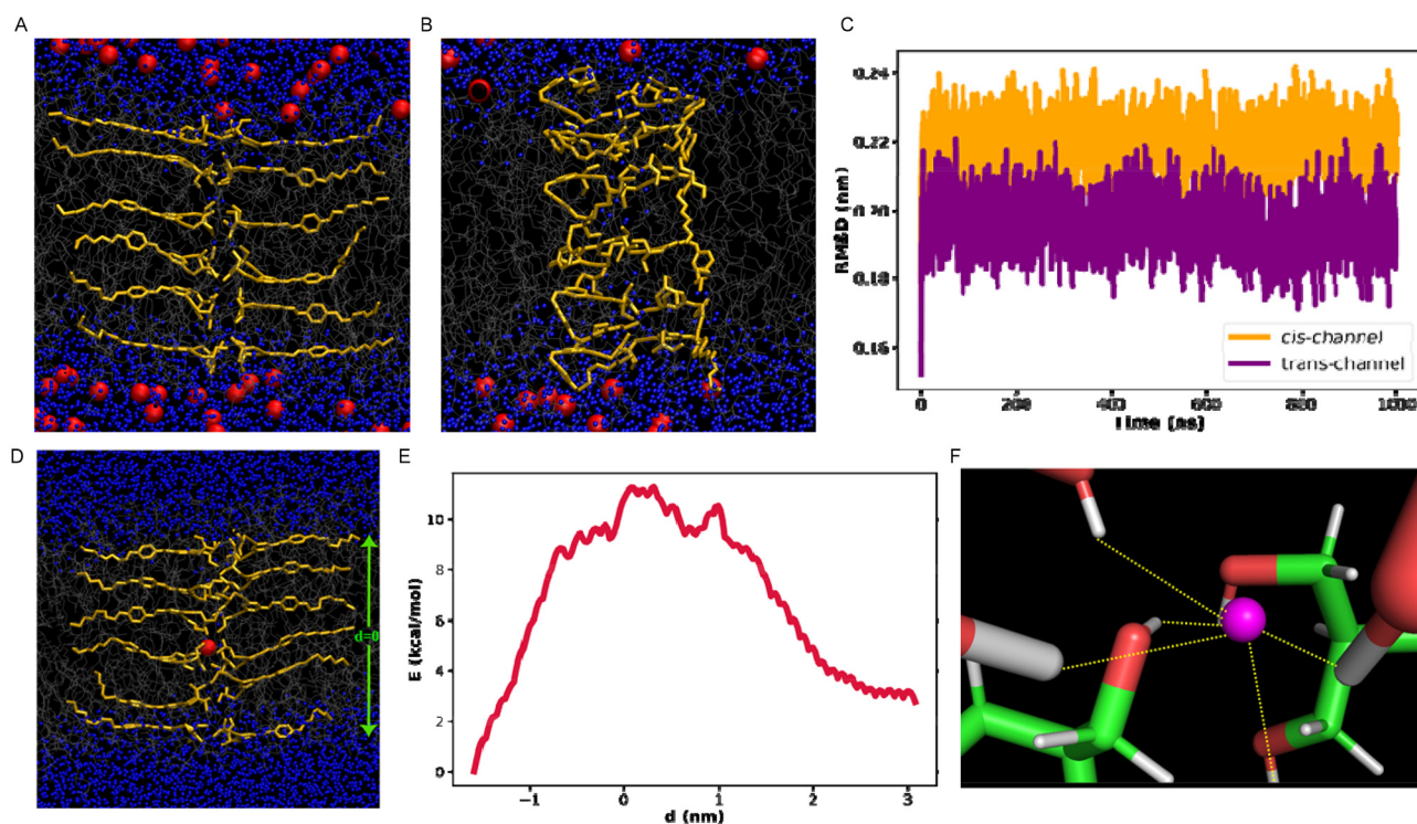
Fig. 5 Representative snapshots of self-assembled 1d , i.e. , trans (A) and the corresponding cis (B) channel structures embedded within the lipid membrane during equilibrium simulation. Time profile of root mean square deviation (RMSD) of both the channels ( cis and trans ) during equilibrium simulation (C). Snapshot of trans channel displaying the collective variable, d , used in umbrella simulation (D) and free energy profile (calculated employing umbrella sampling simulation) of the \text{Cl}^- transport through the more stable trans channel represented corresponding to cv and d (E). The possible interactions between the \text{Cl}^- ion and the channel residues within the trans channel during ion progression (F).
