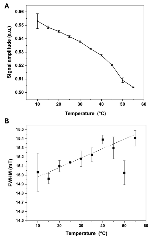
Fig. 8 (A) MPI signal amplitude and (B) FWHM of ferucarbotran (100 \mu\text{g} Fe per mL) at different temperatures ( 10 – 55 ^{\circ}\text{C} ). Data are shown as mean \pm SD for three independent experiments.
