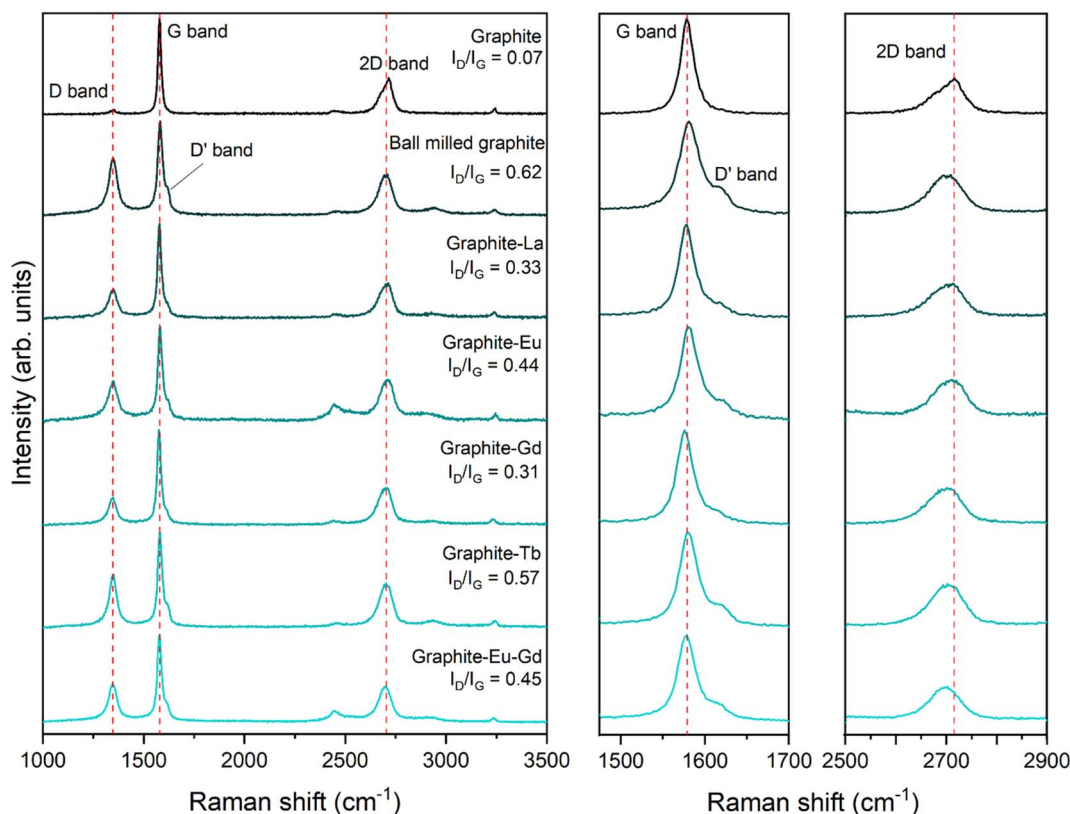
Fig. 5 Comparison of Raman spectra of pristine graphite, ball milled graphite, and graphite-Ln nanocomposites.
