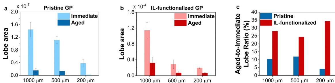
Fig. 4 Comparative analysis of the lobe area and temporal evolution of pristine and IL-functionalized geopolymer devices across varying diameters (1000 μm, 500 μm, 200 μm); (a) and (b) lobe areas measured immediately after fabrication and after one week of aging for pristine and IL-functionalized devices. Error bars represent the standard error of the population; (c) ratio of aged-to-immediate lobe area (%) for pristine and IL-functionalized devices, demonstrating enhanced temporal longevity in IL-functionalized devices.
