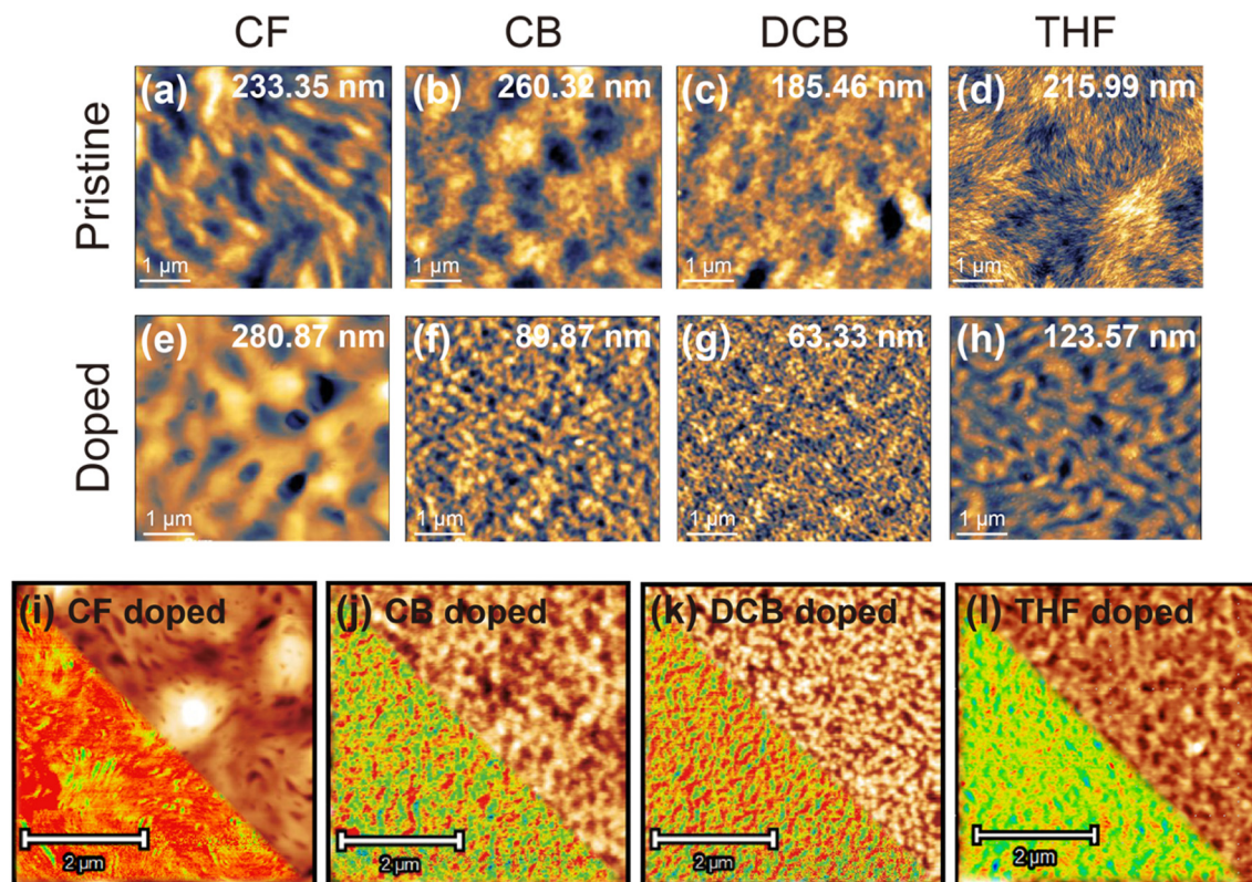
Fig. 6 AFM topography images of (a)–(d) pristine and (e)–(h) TBAF-doped 2PyDPP-2CNTVT films. Images correspond to selected samples with a 35 mol% of TBAF. Correlation lengths are shown at the top of each image. (i)–(l) Topography images with a bottom inset of chemical composition using AFM-IR. Red scale probes a characteristic peak at 1380\text{ cm}^{-1} that is present in the TBAF spectrum. Measurements were performed in tapping mode.
