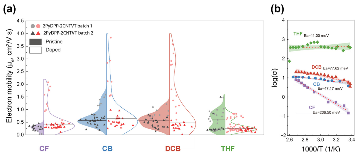
Fig. 7 (a) Violin plots illustrating the distribution of \mu_{\text{e},\text{r}} in pristine (left) and 0.6 mol% TBAF doped (right) 2PyDPP-2CNTVT films processed with various solvents. (b) Temperature dependence of \sigma for 35 mol% TBAF doped 2PyDPP-2CNTVT films processed with CF, CB, DCB, and THF. The different slope for the linear fitting indicates variation in the E_{\text{a}} with 95% confidence band.
