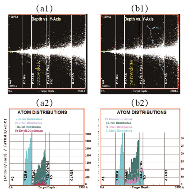
Fig. 5 Ion tracking of 1 MeV H^+ projecting into the (a1) Sn–Pb and (b1) pure Pb PSCs, and the corresponding atomic recoil distributions, (a2) and (b2).
