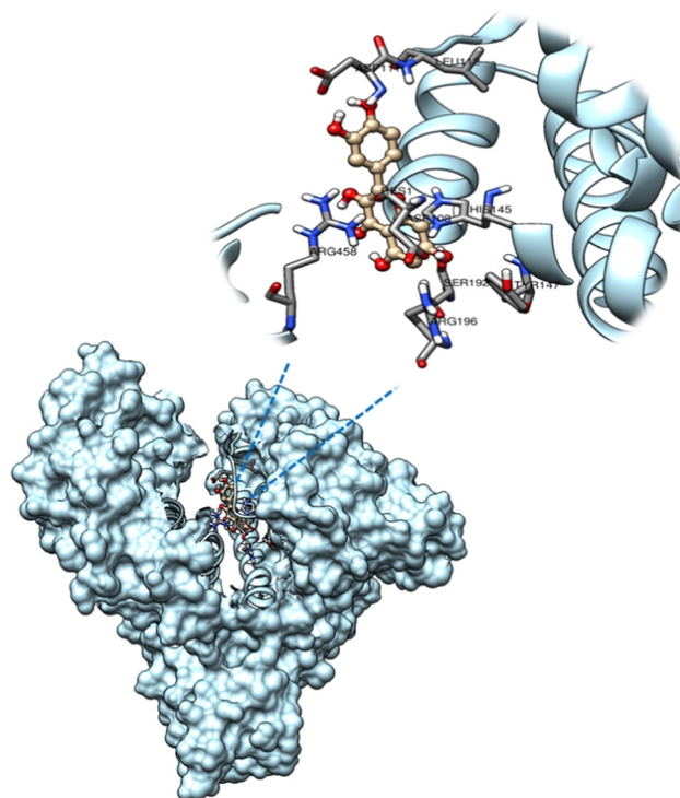
Fig. 12 Molecular docking results of querceetin (wheat, sticks) in BSA (light blue, cartoon). Key interacting amino acid residues are labeled (for clarity, only the chain A is shown).
