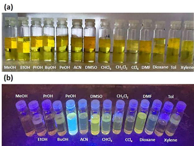
Fig. 13 Fluorescence images of Schiff base ( L 30 ) in different solvents: (a) Normal light (no emission), (b) upon UV radiation (emission wavelength, \lambda_{\text{ex}} = 366 nm) at room temperature; reproduced from ref. 123 with permission from Elsevier, Copyright 2024.
