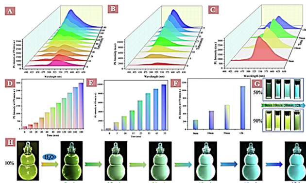
Fig. 12 Changes in fluorescence spectra and intensity of L 26 in THF/H 2 O at 470 nm in THF/H 2 O mixtures with different water fractions of 10% (A) and (D), and 50% (B) and (E), respectively. (G) Changes in emission images of L 26 with time for the 50% and 90% samples. (H) The emission images change of L 26 ( 10^{-4} M in 10% THF/H 2 O) mixtures with different time intervals at an excitation wavelength of 370 nm, and excitation wavelength of 370 nm UV; reproduced from ref. 121 with permission from Elsevier, Copyright 2021.
