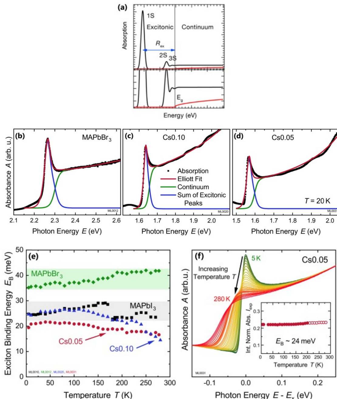
Fig. 2 (a) An example of band-edge absorption spectrum based on eqn (9). The lowest first, second, and third exciton states are approximated with arbitrary broadening which saturates into the continuum near the band-edge. The exciton binding energy is the difference in energy between the free carrier absorption edge and the first exciton peak. The red curve represents the absorption spectrum of free carriers while neglecting the excitonic effects. A magnified image is shown below the main graph. Reprinted with permission, 164 Copyright 2018, American Chemical Society. (b)–(d) Absorption spectra at 20 K as a function of photon energy for MAPbBr 3 , Cs 0.01 FA 0.765 MA 0.135 Pb(I 0.765 Br 0.235 ) 3 (depicted as Cs0.10), and Cs 0.05 (FA 0.83 MA 0.17 ) 0.95 -Pb(I 0.83 Br 0.17 ) 3 (depicted as Cs0.05) respectively. The red line represents Elliott's fit while the green and blue lines correspond to excitons and continuum contribution. (e) Estimation of exciton binding energy E_{xb} for MAPbI 3 , MAPbBr 3 , Cs 0.01 , and Cs 0.05 according to the absorption spectra of (b, c, d). (f) Normalized spectra for Cs 0.05 from 5 K to 280 K with respect to energy shift by excitonic peak E_x whereas the inset represents the integrated normalized spectra I_{exp} . Adapted from ref. 97, Copyright 2019, American Institute of Physics.
