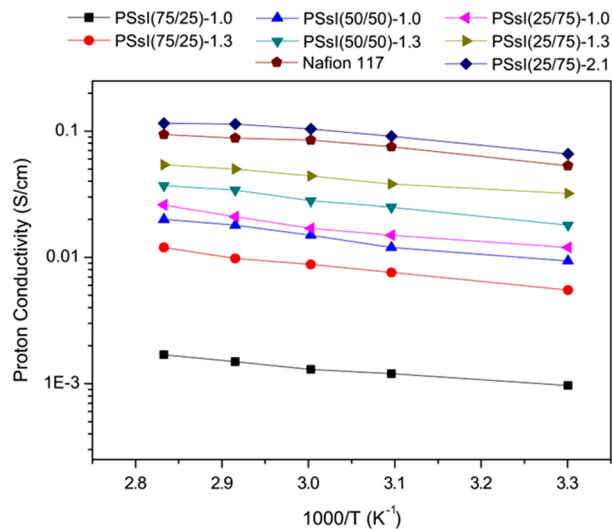
Fig. 20 Arrhenius plot of proton conductivity of Nafion-117 and PSsI membranes at 100% RH. Reprinted with permission from ref. 168. Copyright Elsevier 2015 (license number: 5677791420578).
