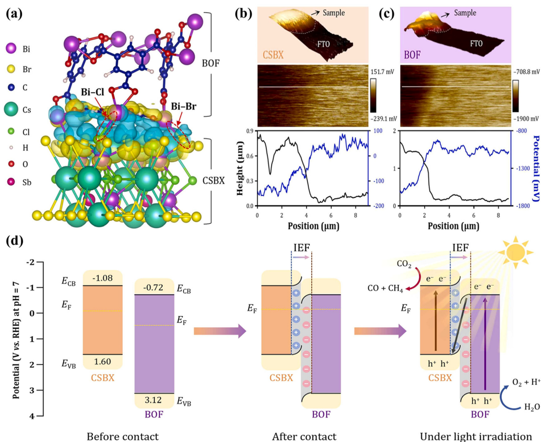
Fig. 5 Lead-free halide-perovskite-based heterojunction: (a) charge density difference (isosurface level, 0.04 e - Å -3 ) over the CSBX/BOF heterojunction. The yellow and cyan regions represent the positive and negative electron density isosurfaces, respectively, KPFM surface potential images (middle), and the corresponding topography and surface potential line profiles (bottom) for (b) CSBX and (c) BOF three-dimensional topographical maps (top). (d) Schematic of the band structures of CSBX and BOF (left), interfacial charge transfer and the formation of an IEF upon hybridisation (middle), and CSBX/BOF S-scheme heterojunction under light irradiation (right). Reproduced from ref. 93, with permission of Applied Catalysis B: Environment and Energy , copyright 2025.
