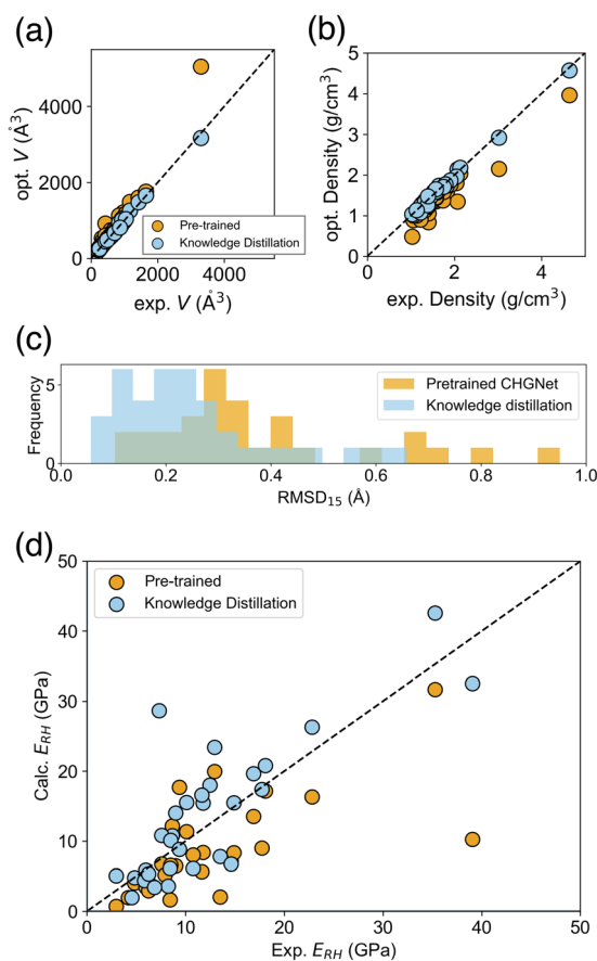
Fig. 7 Observed–predicted plot of elasticity dataset using pretrained and knowledge distillation models. The metrics of (a) cell volume, (b) crystal density, and (c) RMSD 15 . (d) The observed–predicted plot of Young's modulus E_{RH} . The dashed lines are the reference lines when predictions perfectly match with experimental data.
