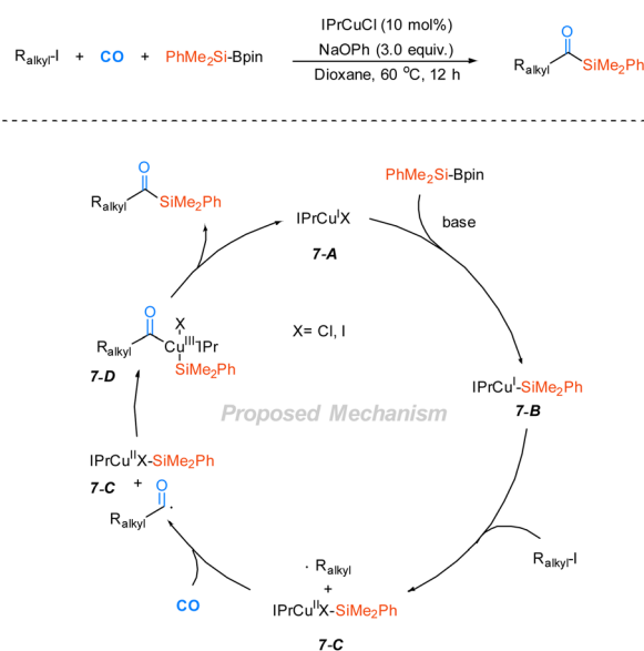
Fig. 7 Copper-silyl intermediate-mediated carbonylation toward acylsilyl-lane derivatives.
