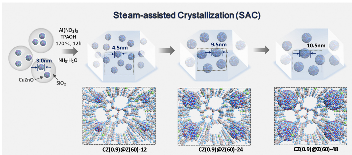
Fig. 1 Schematic of CZ(0.9)@Z- t preparation at different crystallization times ( t = 12, 24, \text{ and } 48 \text{ h} ).
