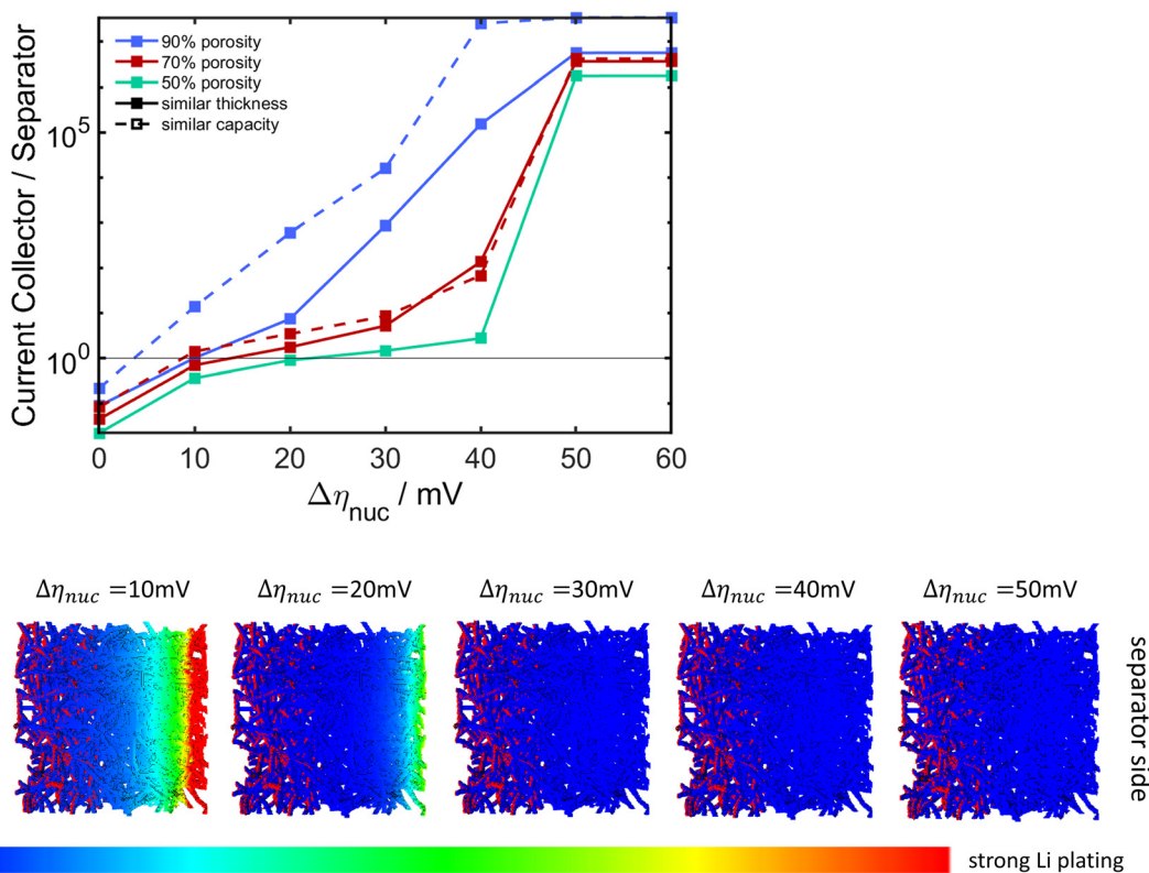
Fig. 6 Top: influence of a gradient in lithiophilicity on the ratio of the effective, mean amount of Li plating on the current collector and separator sides of different porous microstructures (train 11 635, train 5481, and train 44 842; cf. Table S3†) with similar thickness and similar capacity after 10 s at 0.1 \text{ mA cm}^{-2} . An extended figure which additionally includes a dual-layer structure with a surface area and porosity gradient can be found in the ESI (Fig. S19†). Bottom: the amount of plated Li on a highly porous (90%) fiber system with different lithiophilicity (train 11 635; cf. Table S3†) in combination with a thin lithiophilic interlayer ( \eta_{\text{nuc}} = 0 \text{ V} ) after 10 s at 0.1 \text{ mA cm}^{-2} . The shown view is from the side in the through direction. The current collector is located on the left side, while the separator is beginning on the right. An extended figure including all three structures with different porosities can be found in the ESI (Fig. S18†).
