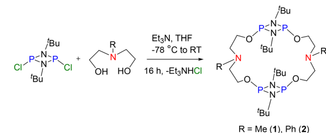
Scheme 1 Synthesis of macrocycles – [[P(\mu-N^tBu)]_2\{O(CH_2)_2N(Me)(CH_2)_2O\}]_2 ( 1 ) and [[P(\mu-N^tBu)]_2\{O(CH_2)_2N(Ph)(CH_2)_2O\}]_2 ( 2 ).
