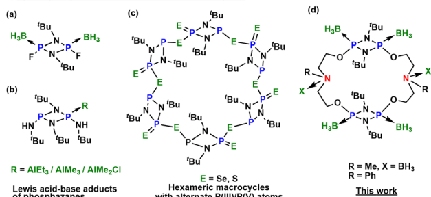
Fig. 1 (a and b) Selected examples of cyclodiphosphazane [P(\mu-N^tBu)]_2 -based adducts with main group Lewis acids; (c) an example of the heteroleptic P^V/P^{III} macrocycle; and (d) the newly synthesized first main group Lewis acid base adduct with phosphazane macrocycles.
