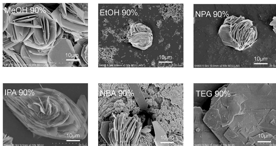
Fig. 3 SEM images of the self-assembled products of \text{In}(\text{NO}_3)_3/S^- in 90 vol% alcohol/ \text{H}_2\text{O} at 100 °C.
