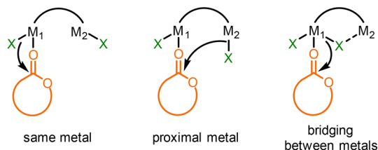
Fig. 6 Potential mechanisms for the initiation of lactide ring-opening polymerisation (where X is a nucleophile such as an alkoxide or a propagating polymer chain).
