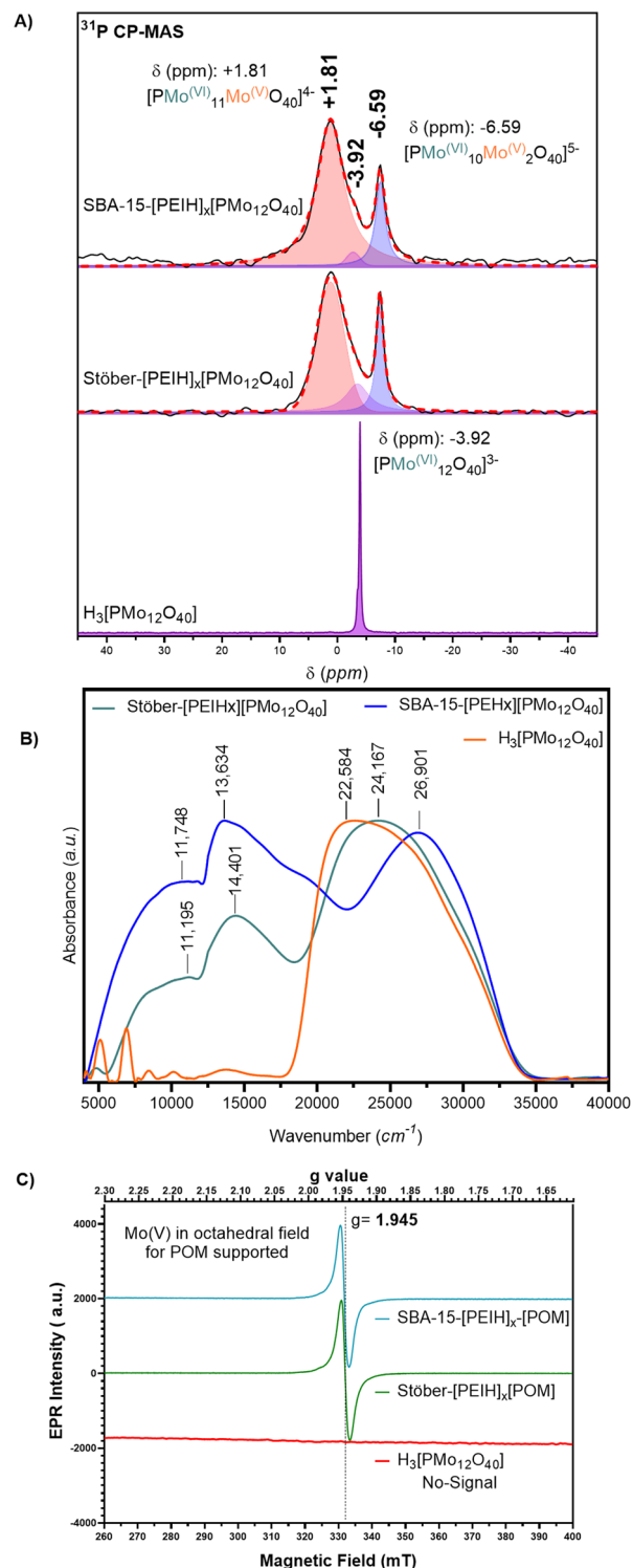
Fig. 4 Spectroscopic characterization of SiO 2 -[PEIH x ][PMo 12 O 40 ]. A) 31 P CP-MAS NMR spectra, B) diffuse reflectance ultraviolet-visible-near infrared spectra, and C) solid state EPR spectra of Mo(V) cations embedded in supported POM clusters at 77 K.
