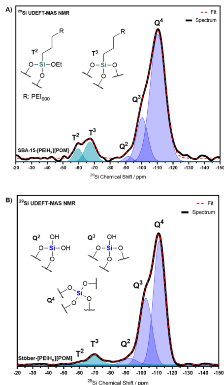
Fig. 3 29 Si UDEFT-MAS NMR spectra of a) SBA-15-[PEIH x ][POM] (A) and Stöber-[PEIH x ][POM] (B), with inset of structures of Si species observed (T n : carbon-bonded silicon atoms, Q n : silanols and siloxanes).
