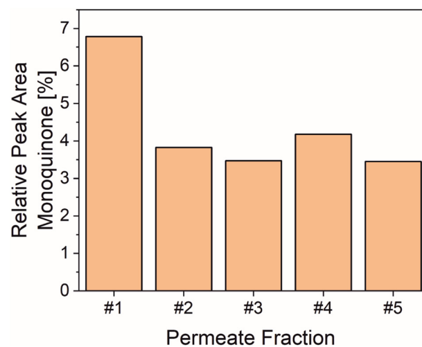
Fig. 3 Extracted HPLC data for the conversion of dihydroxytyrosine by immobilized SinATyr in flow mode. The peak areas for the substrate dihydroxytyrosine and the monooxidation product (= monoquinone) within the respective chromatogram for each of the collected permeate fractions were detected and summed up. The peak area portion for the monoquinone with respect to this sum is then plotted ("Relative Peak Area Monoquinone"). Each fraction had a volume of 500 \mu\text{L} and the flow rate was set to 50 \mu\text{L min}^{-1} . The amount of immobilized enzyme was 11.4 \mu\text{g} and substrate concentration was set to 1 mM (50 mM sodium citrate buffer, pH 6.8).
