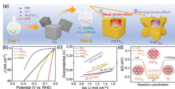
Fig. 1 (a) The synthesis schematic illustration of \text{PdPt}_2\text{L} and \text{PdPt}_2\text{M} . (b) LSV polarization curves between Pd, \text{PdPt}_2\text{L} , \text{PdPt}_2\text{M} , and commercial Pt/C. (c) Tafel slopes. (d) \Delta G_{\text{H}^*} on Pt sites of \text{PdPt}_2\text{L} and \text{PdPt}_2\text{M} , and Pt. The insets are atomic structure simulation model of \text{PdPt}_2\text{L} , \text{PdPt}_2\text{M} , and Pt with adsorbed hydrogen. 54
