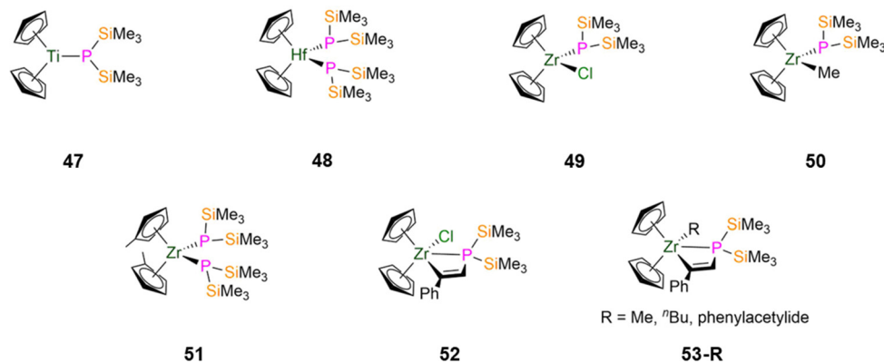
Fig. 14 Group 4 P'' complexes [Ti(Cp)_2(P'')]_2 ( 47 ), [Hf(Cp)_2(P'')]_2 ( 48 ), [Zr(Cp)_2(Cl)(P'')]_2 ( 49 ), [Zr(Cp)_2(Me)(P'')]_2 ( 50 ), [Zr(C_5H_4Me)_2(P'')]_2 ( 51 ), [Zr(Cp)_2(Cl)(P(SiMe_3)_2C(H)C(Ph))]_2 ( 52 ), [Zr(Cp)_2(R)(P(SiMe_3)_2C(H)C(Ph))]_2 ( 53-R ; R = Me, n Bu, C \equiv CPh).
